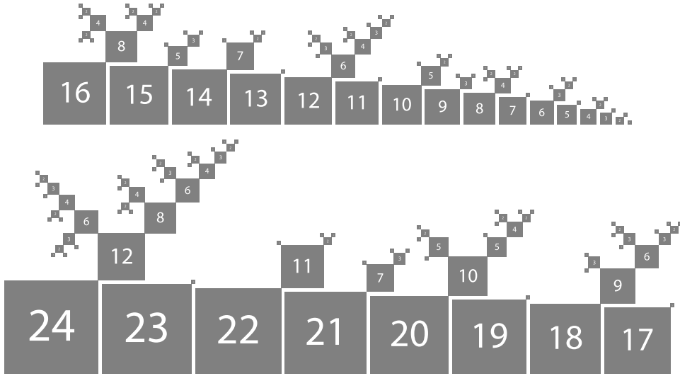
Fig. 1. Divisor trees for 1 to 24. The number of recursive divisors \kappa_0(n) counts the number of squares in each tree. The sum of recursive divisors \kappa_1(n) adds up the side length of the squares in each tree. The sum of the square of recursive divisors \kappa_2(n) adds up the area in each tree, and so on.
