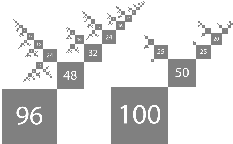
Fig. 2. Divisor trees for 96 and 100. There are \kappa_0(96) = 224 squares in the left tree and \kappa_0(100) = 52 squares in the right tree. The sum of the side length of the squares, or one-fourth of the tree perimeter, is \kappa_1(96) = 768 and \kappa_1(100) = 340 . The sum of the area of the squares is \kappa_2(96) = 16,608 and \kappa_2(100) = 14,740 .
