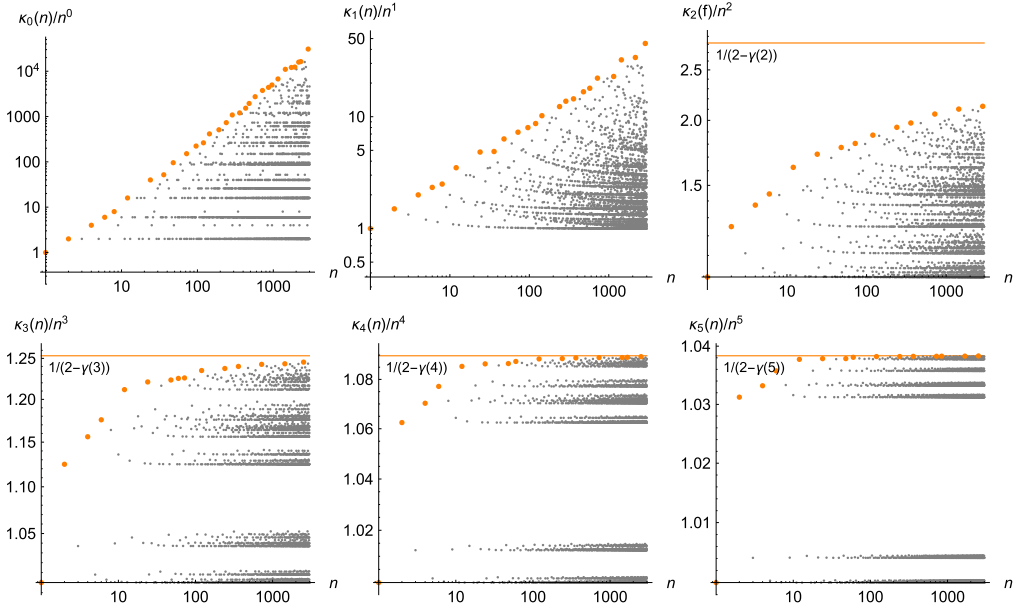
Fig. 3. Plots of \kappa_x(n)/n^x . We plot \kappa_x(n)/n^x up to n = 3,000 , for x = 0 to x = 5 . The large points (which are orange in the online version) are the sequence records, which satisfy \kappa_x(n)/n^x > \kappa_x(m)/m^x for all m < n . For x = 0 and x = 1 , the upper bound for the sequence diverges. But for x = 2 and above, it converges to 1/(2 - \gamma(x)) , where \gamma is the Riemann zeta function. For x = 0 , the large points are the recursively highly composite numbers. For x = 1 , they are the recursively super-abundant numbers (see Appendix A).
