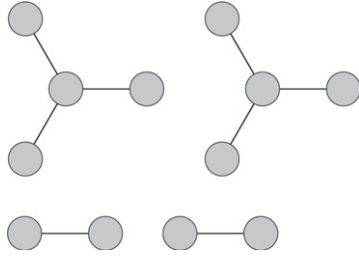
Figure B1. A validation example with nonconstant degree-degree correlation.
